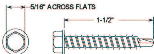
#14-13 X 1-1/2" Screw Mini-point Hex Washer Head
