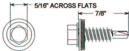
1/4-14 X 7/8" Hex Washer Head (HWH) Stitch Screw w/Grommated Washer, Mill Point Metal to Metal (Max. 18 ga. Panel)
