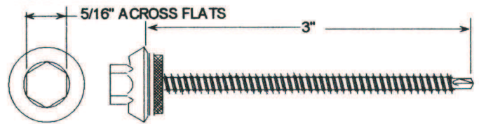
#12-14 X 3" Hex Washer Head (HWH) Screw W/Grommated Washer Mill Point Metal to Metal (Max. 18 ga. Panel)
