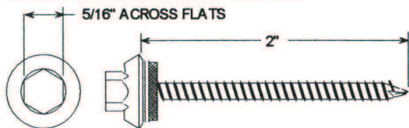
#10-16X 2" Hex Washer Head (HWH) Screw W/Grommated Washer A/B Point Metal to Wood
