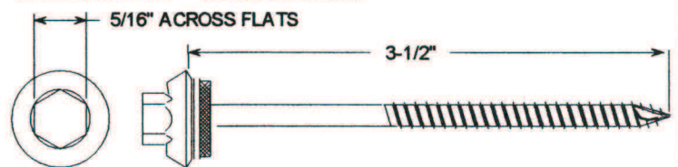
#14-10X 3.5" Hex Washer Head (HWH) Screw, W/Grommated Washer, Type 17 Point, Metal to Wood
