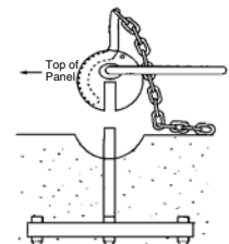
T-90-F Face Lift Insert (Shown with optional T-90-C Floating Rebar Clip)
