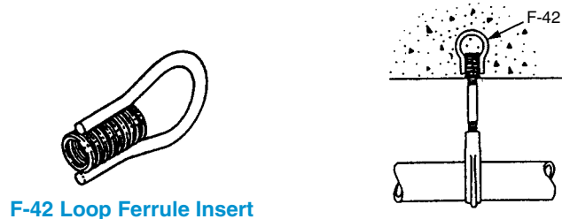
F-42 Loop Ferrule Insert
