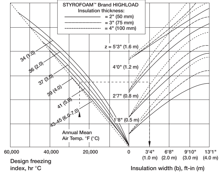
Figure 3: Sand or Gravel – Inverted “U” Insulation
