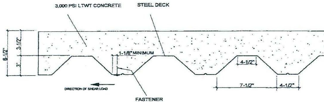
SECTION – COMPOSITE DECK – NO SCALE
