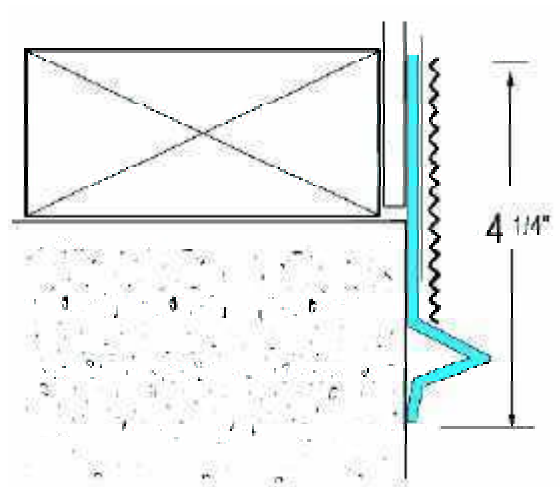
Foundation Weep Screed
