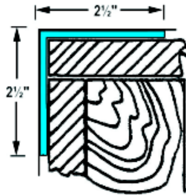
EIFS Corner Bead
