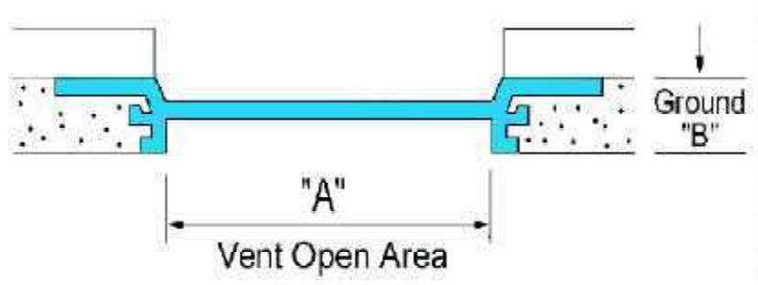
Vinyl Soffit Screed
