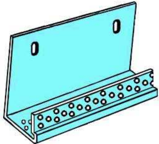
EIFS Starter Track Casing Bead with Drainage Holes
