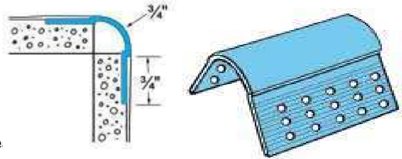
Drywall Bull Nose Corner Be
