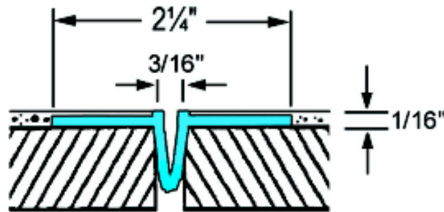
EIFS 1/16" Expansion Joint
