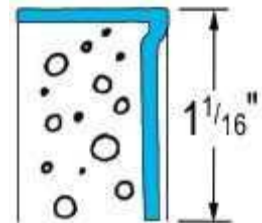
Drywall "MJ" Bead
