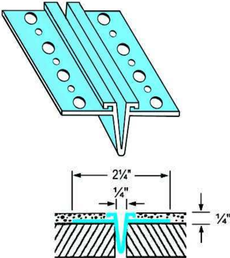
EIFS 1/4" Expansion Joint
