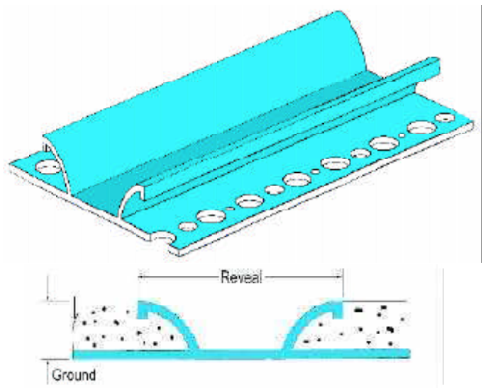
Vinyl Stucco Bull Nose Reveal
