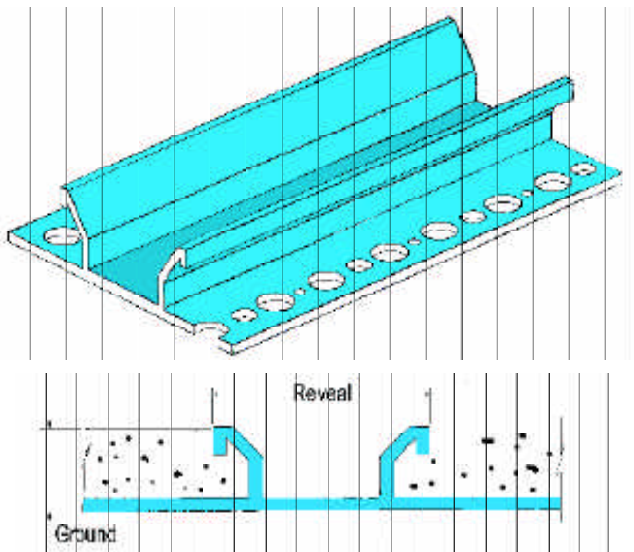
Vinyl Stucco Chamfered Reveal
