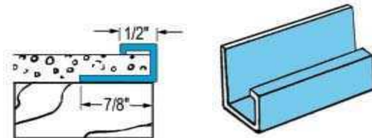
Drywall Shadow Line "J" Bead
