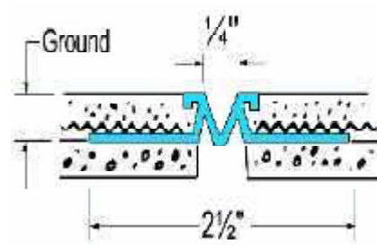
Vinyl Control Joint
