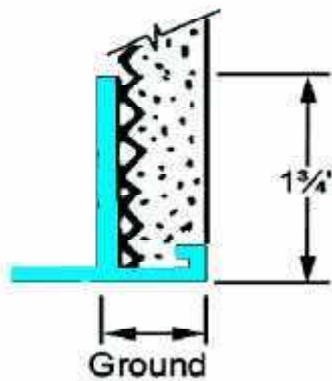
Vinyl Casing Bead with Reveal
