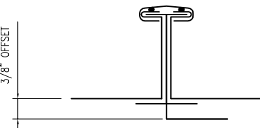
AFTER SEAMING
