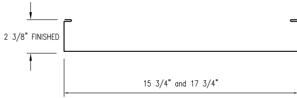
238T PANEL PROFILE Standard Width(s)- 15 3/4" and 17 3/4"
