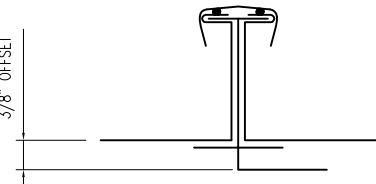
BEFORE SEAMING
