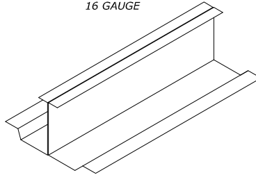
CONTINUOUS CLIP 2-PIECE
