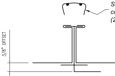
SEAM ENGAGEMENT
