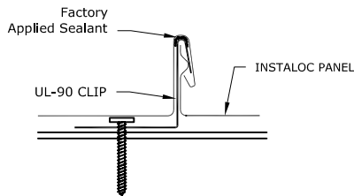
INSTALOC PANEL SEAM
