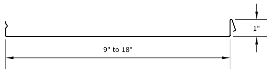
INSTALOC PROFILE (SMOOTH) Standard Width(s)- 13" and 18"
