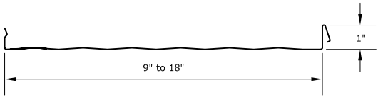
INSTALOC PROFILE (STRIATIONS) Standard Width(s)- 13" and 18"
