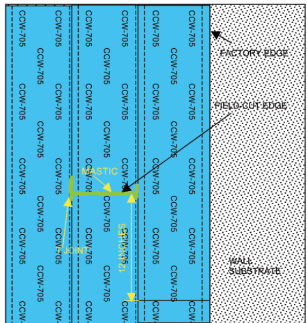
Figure 2: Installation in Vertical Runs
