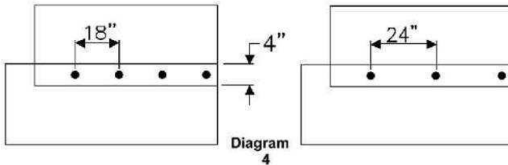
Attachment of base sheet using Firestone MB 2" Barbed Metal Lap Plates and Fasteners 4" = 101.6 mm 18" = 457.2 mm 24" = 609.6 mm
