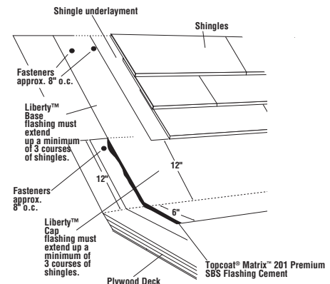
Shingle Tie-In
