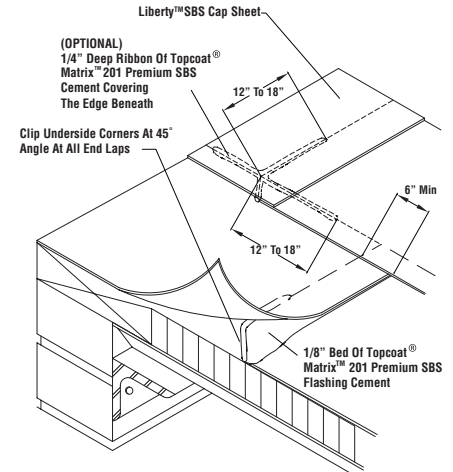
Figure 3-1 (End Lap)
