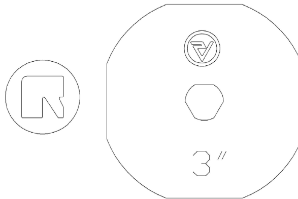
FIGURE 1—HEAD AND WASHER MARKINGS
