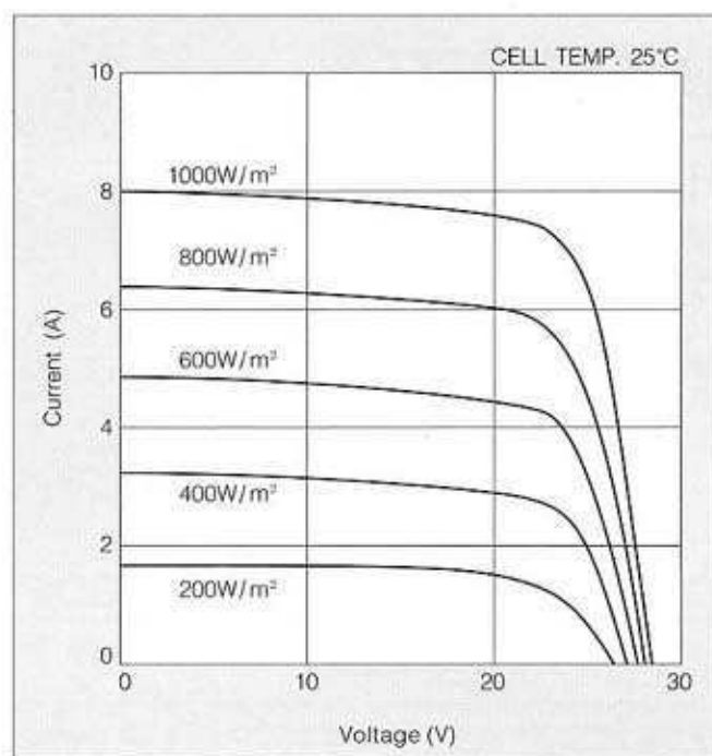
Current-Voltage characteristics of Photovoltaic Module KC167G at various irradiance levels
