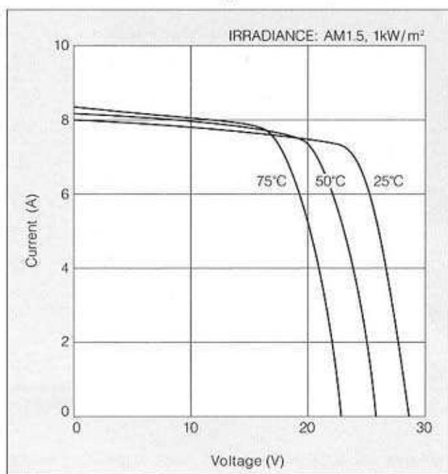
Current-Voltage characteristics of Photovoltaic Module KC167G at various cell temperatures
