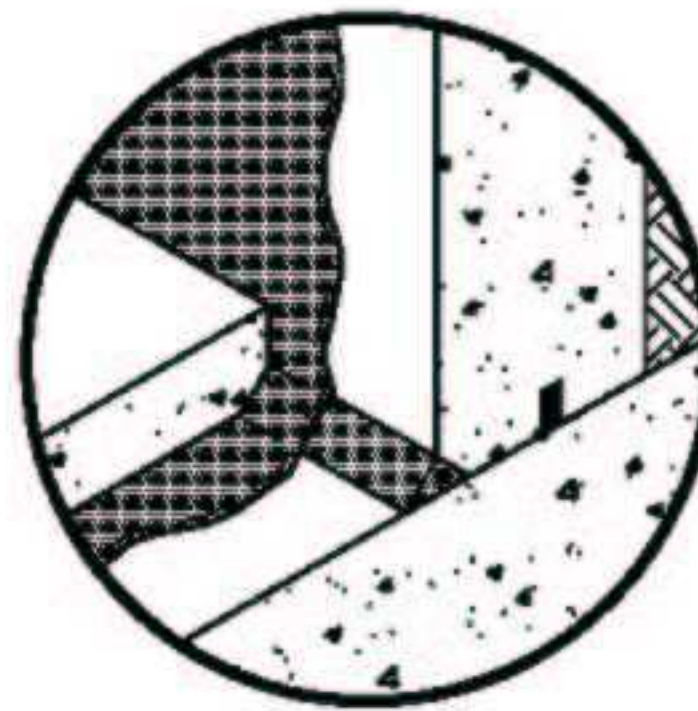
ALTERNATE CORNER DETAIL FOR CRYSTALLINE WATERPROOFING
