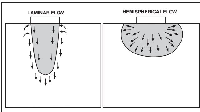
Figure 22. Laminar Flow Diffusion Pattern
