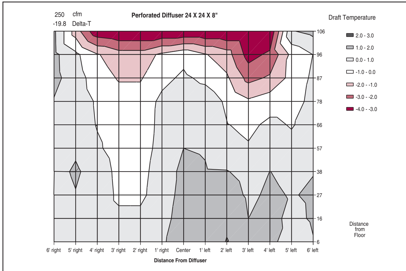
Figure 37. Room Isodrafts
