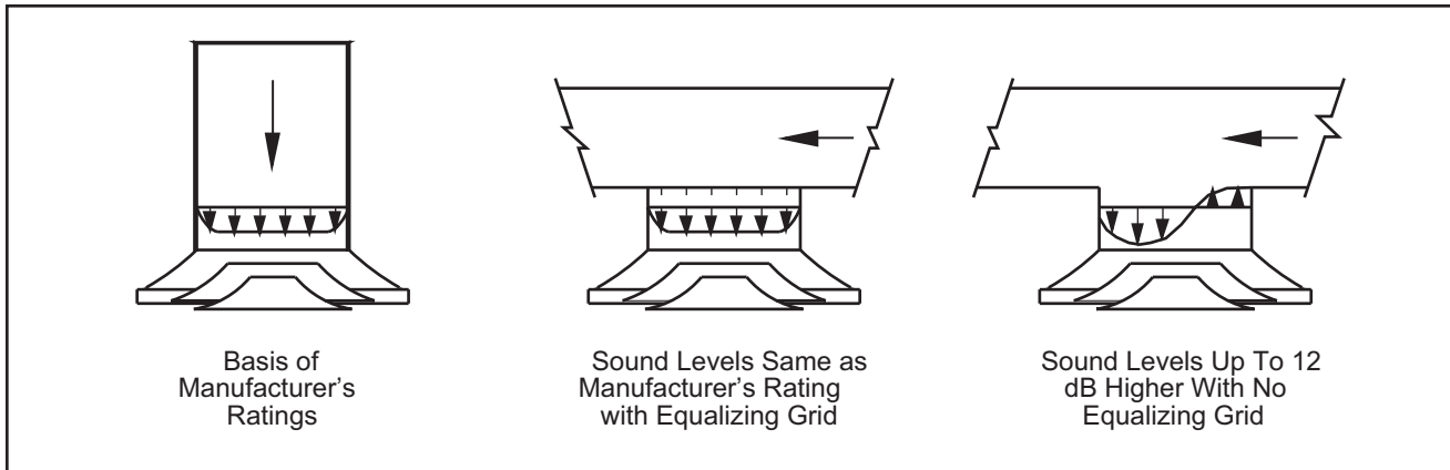
Figure 45. Equalizing Grid Effects (from ASHRAE Standards Handbook; Atlanta, GA)
