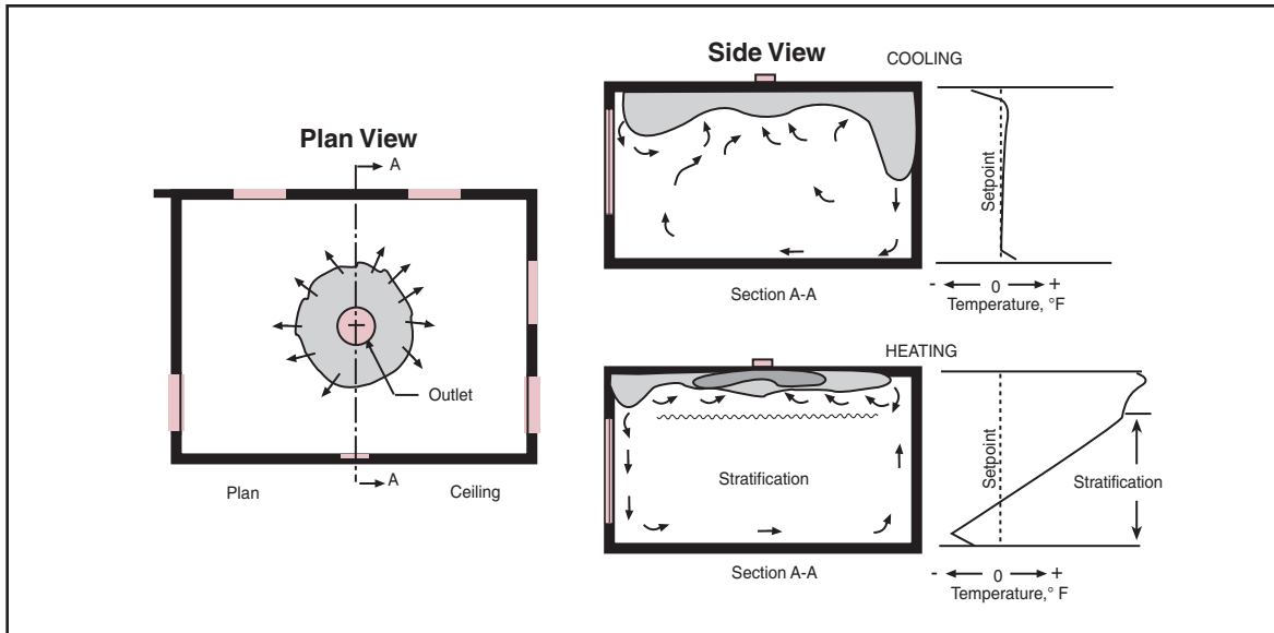
Figure 18. Circular Horizontal Air Projection at the Ceiling Level
