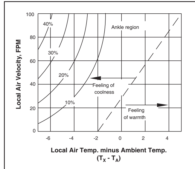
Figure 2. Comfort Chart - Ankle Region
