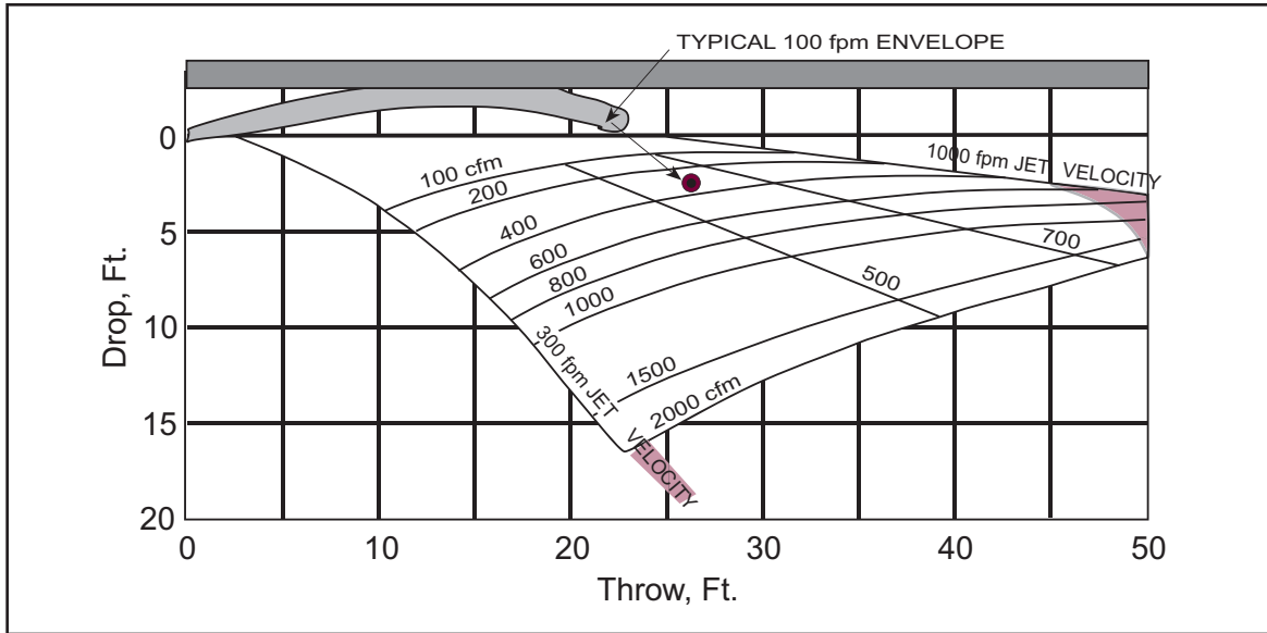
Figure 10. Throw and Drop for Outlet 2-4 feet Below Ceiling, 20 Degrees Vertical Deflection, 0 Degrees Spread
