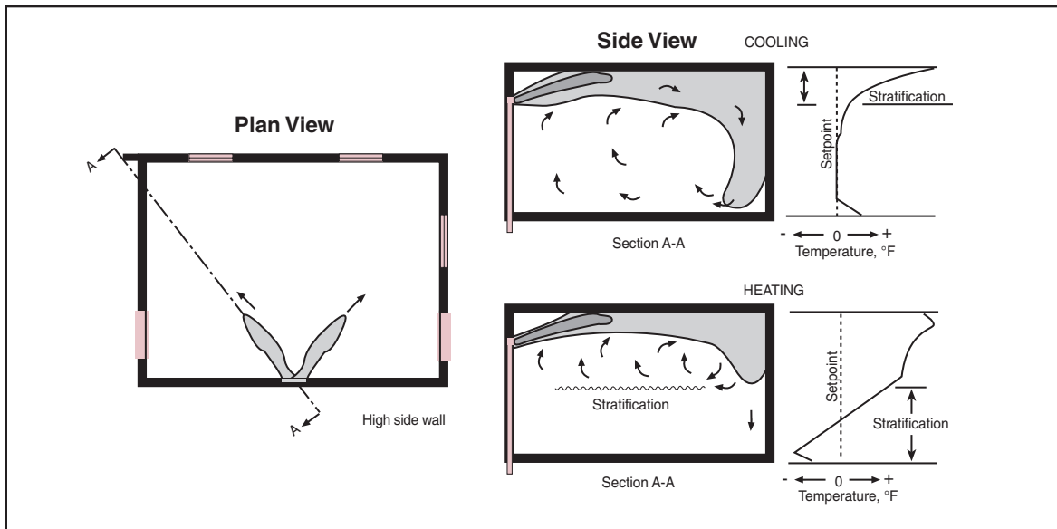
Figure 17. Spreading Horizontal Air Projection at the Ceiling Level
