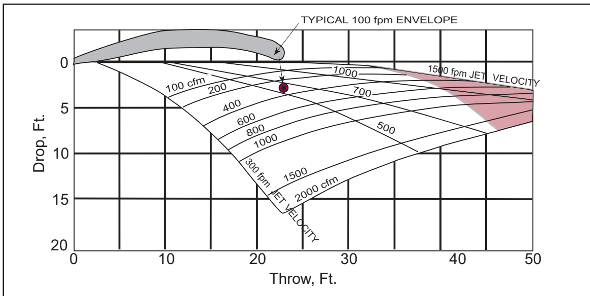
Figure 11. Throw and Drop for Outlets Mounted Without Ceiling, 20 Degree Vertical Deflection, 0 Degree Spread
