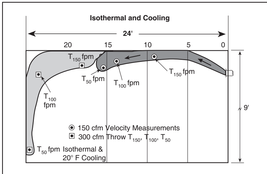
Figure 9. Mapping of Cooled Air Throw
