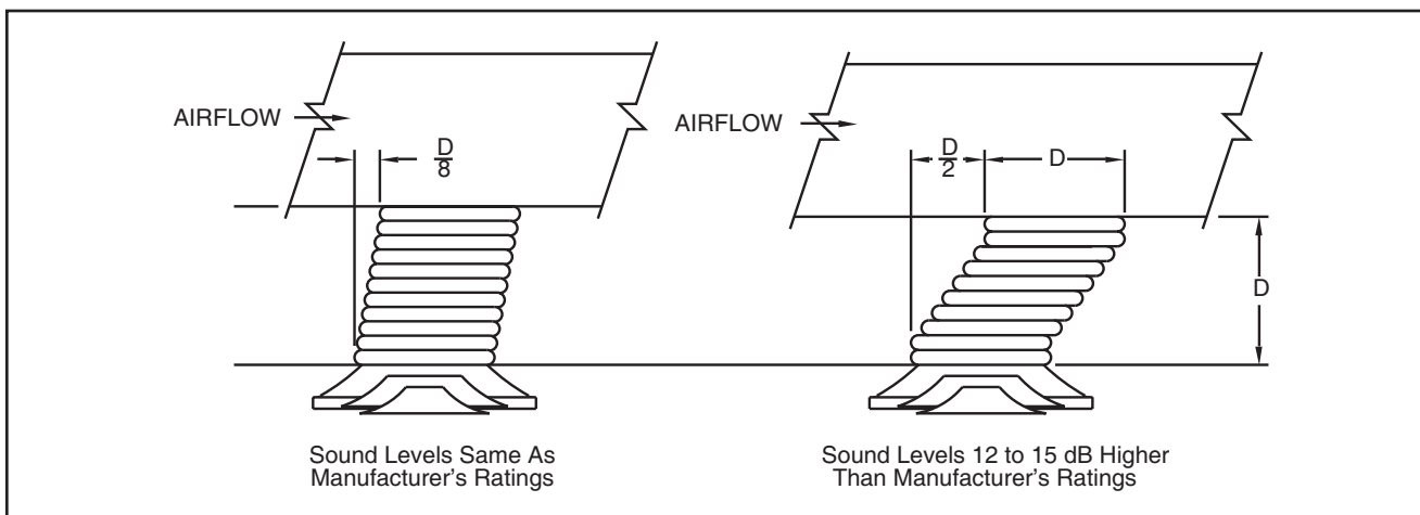
Figure 46. Flexible Duct Inlet Effects (from ASHRAE Standards Handbook; Atlanta, GA)
