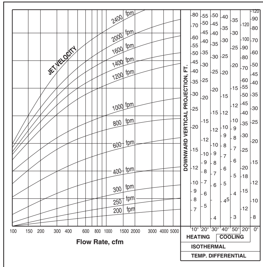
Figure 24. Downward Vertical Projection
