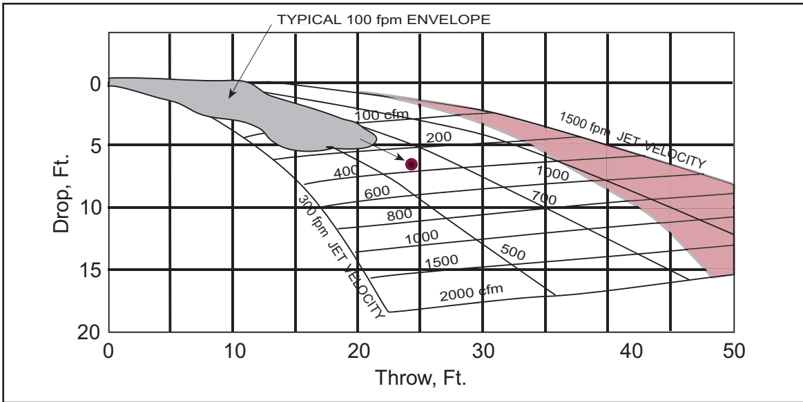
Figure 13. Throw and Drop for Outlet Without Ceiling, 0 Degree Deflection, 0 Degree Spread
