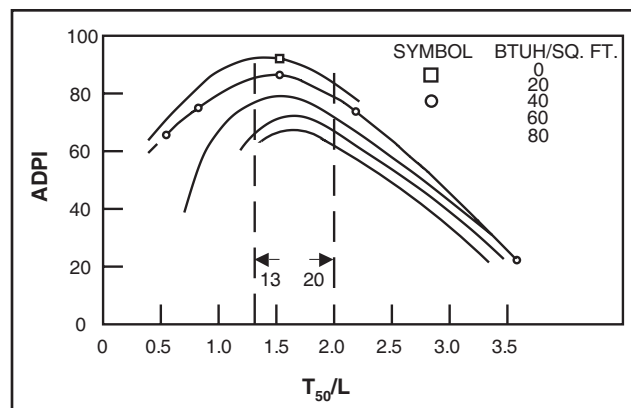
Figure 38. ADPI vs. T_{50}/L for High Side Wall Grilles (from Kansas State University tests)
