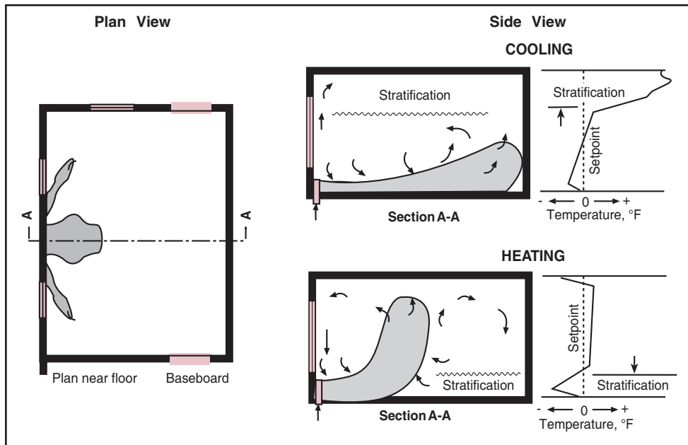
Figure 27. Schematic of Displacement Ventilation
