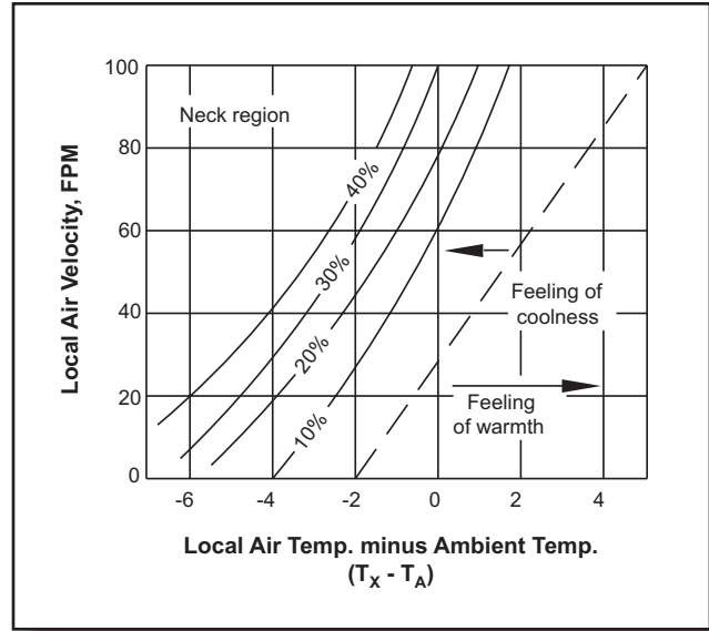
Figure 1. Comfort Chart - Neck Region
