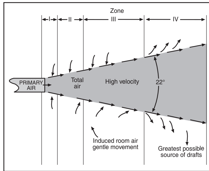
Figure 6. Expansion of primary air jet
