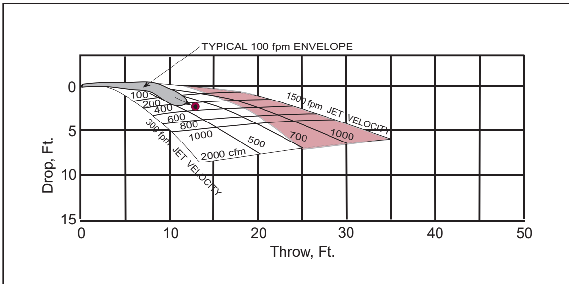
Figure 15. Throw and Drop for Outlet 2 to 4 Feet Below Ceiling, 0 Degree Vertical, 45 Degree Spread
