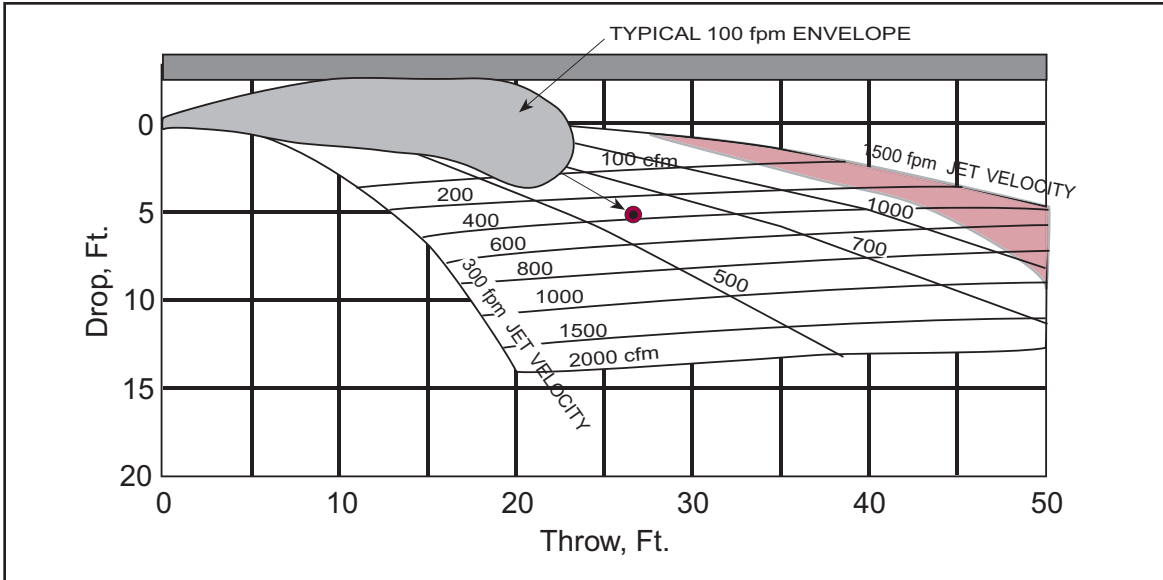
Figure 12. Throw and Drop for Outlet 1 Foot Below Ceiling 0 Degree Deflection, 0 Degree Spread
