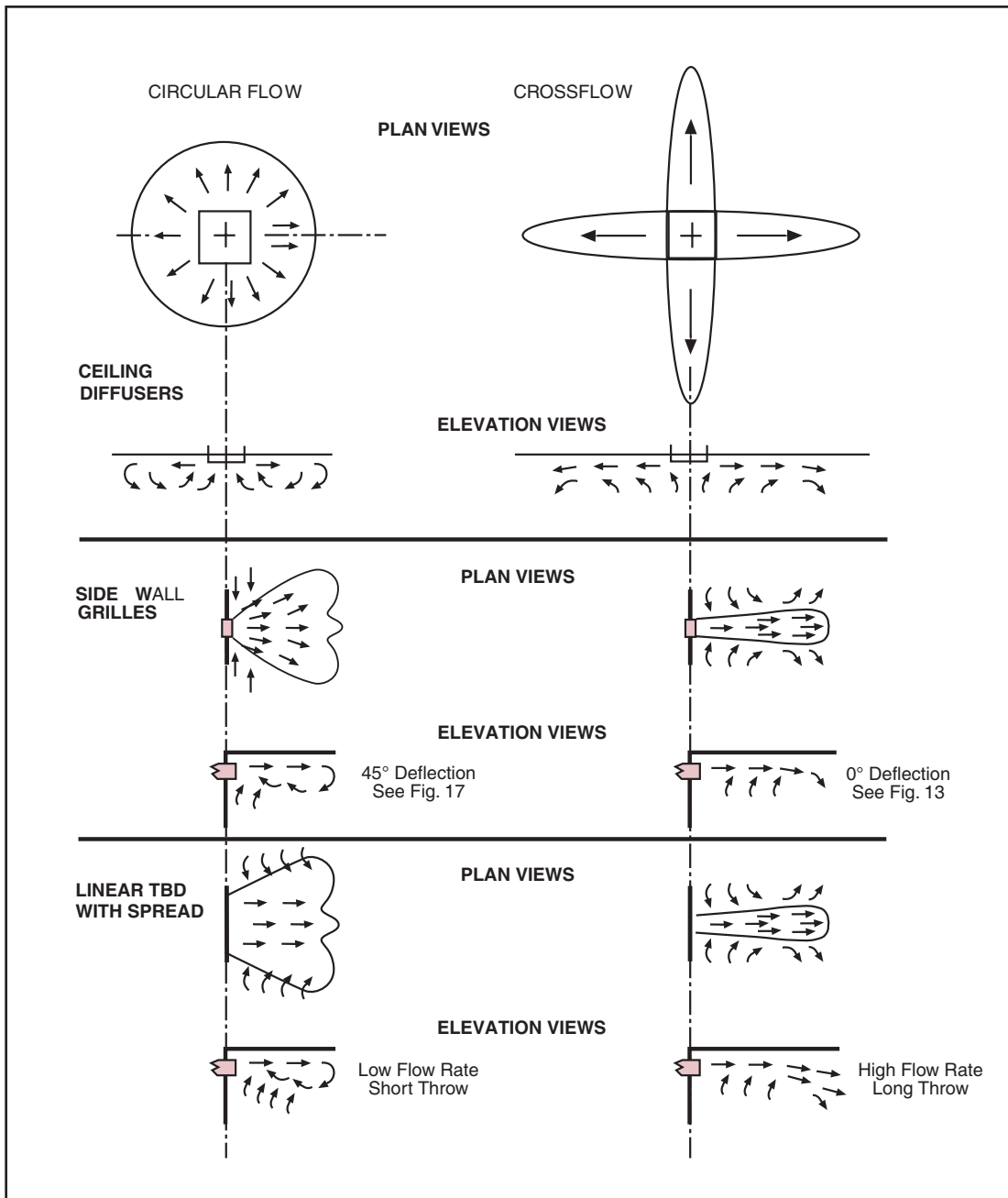
Figure 19. Some Specific Airflow Characteristics at High and Low Airflow Rates
