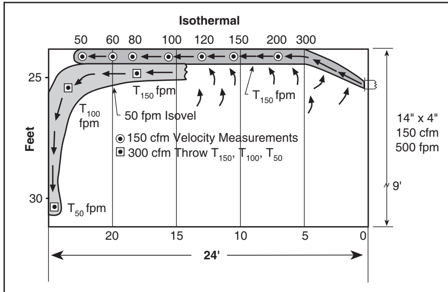
Figure 8. Mapping of Isothermal Throw
