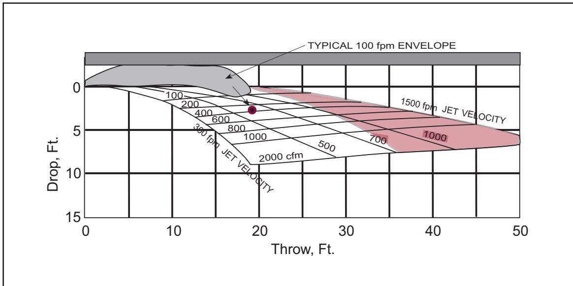
Figure 14. Throw and Drop for Outlet 1-1/2 Feet Below Ceiling, 0 Degree Vertical, 45 Degree Spread
