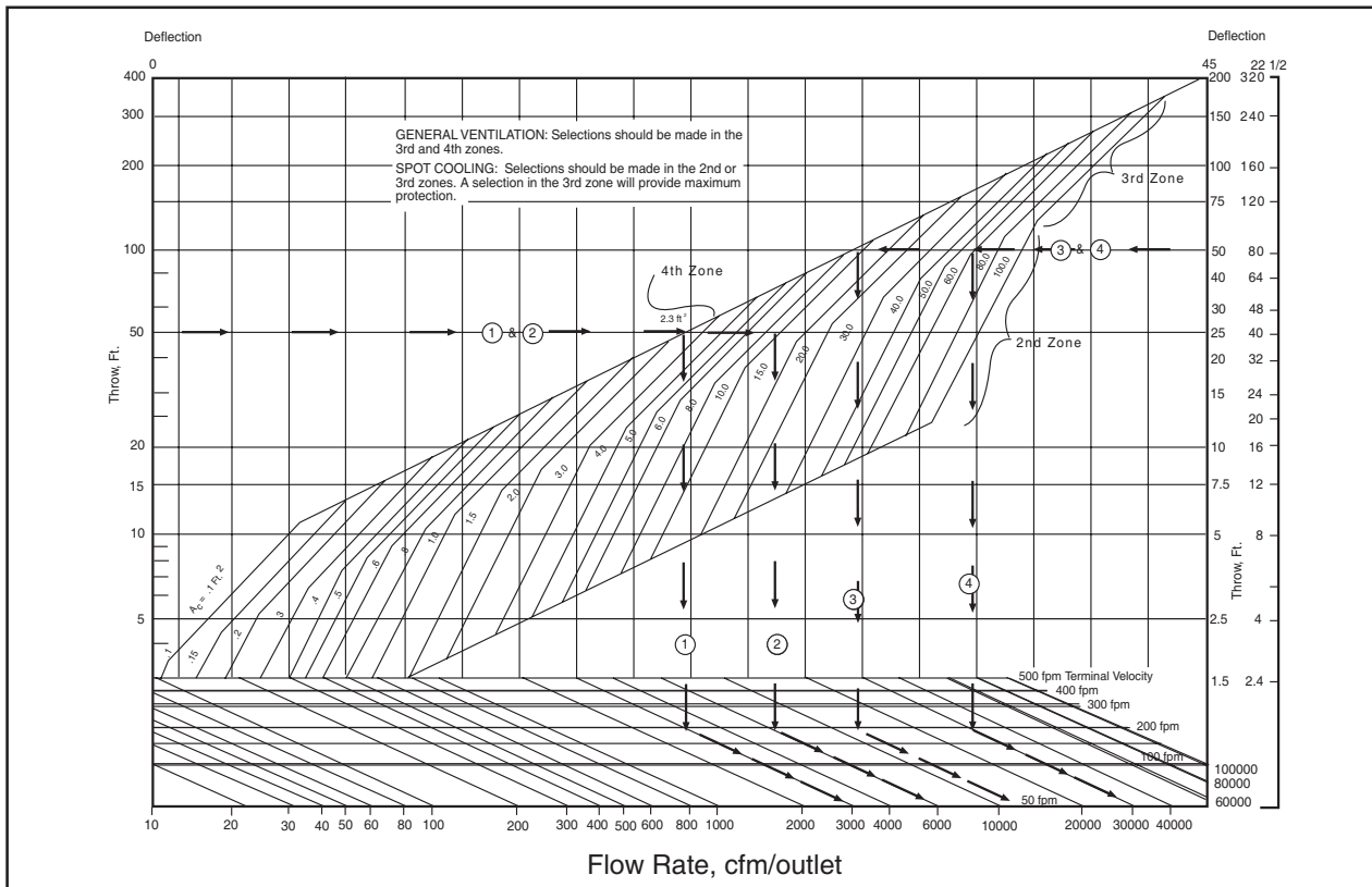
Figure 41. Grille Selection Chart for Industrial Applications
