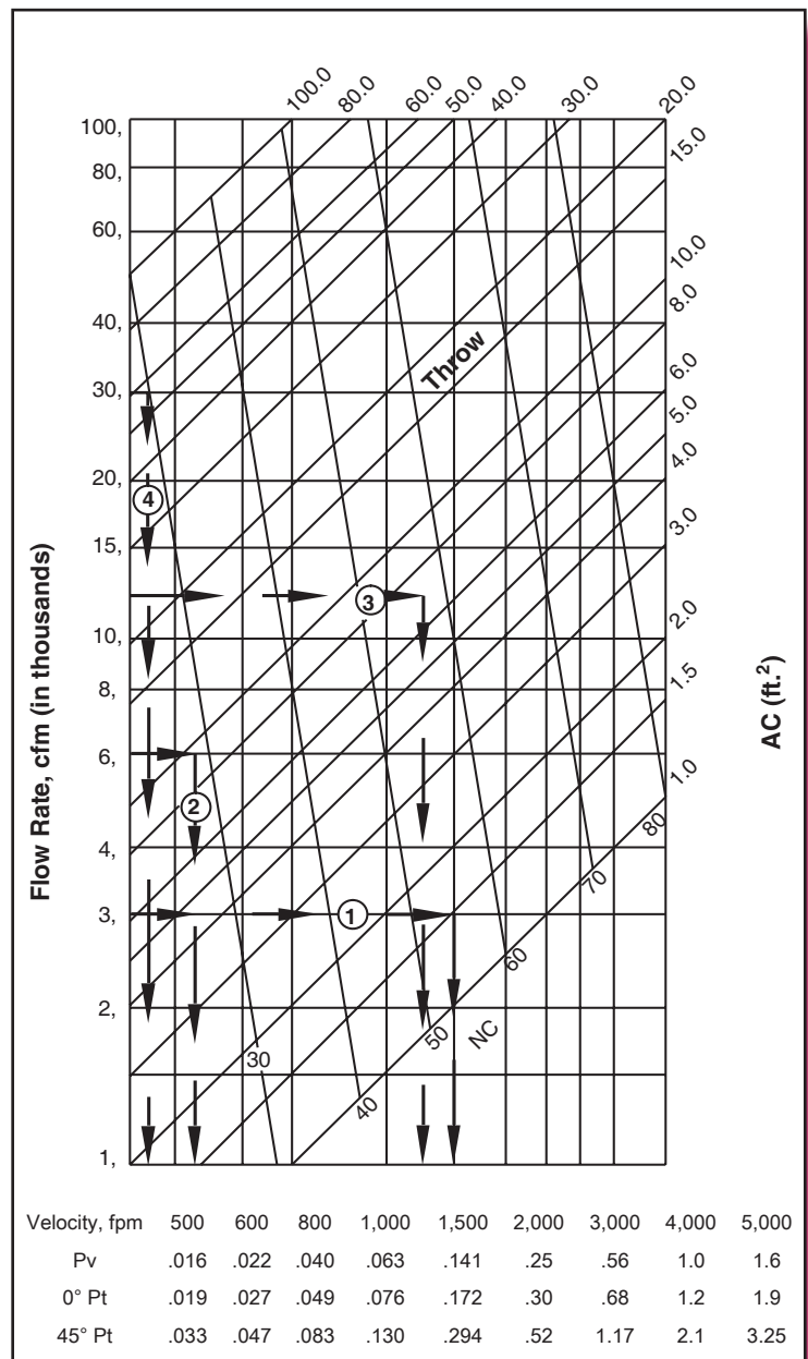
Figure 42. Typical Sound and Pressure Drop for Grilles
