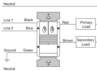
PW-200 Dual Circuit Wiring
