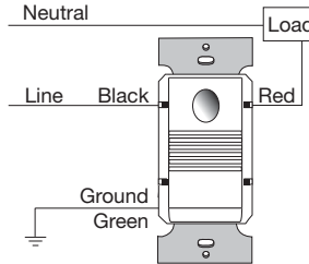
PW-100 and PW-100-347 Wiring
