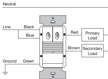
PW-200 Bi-Level Wiring
