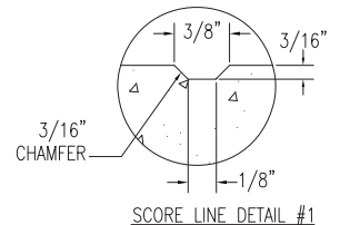
SCORE LINE DETAIL #1
