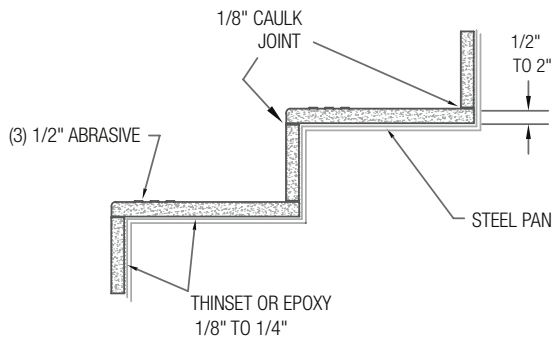
TT2000™ SERIES E-40 EPOXY TERRAZZO SEPARATE TREAD AND RISER
