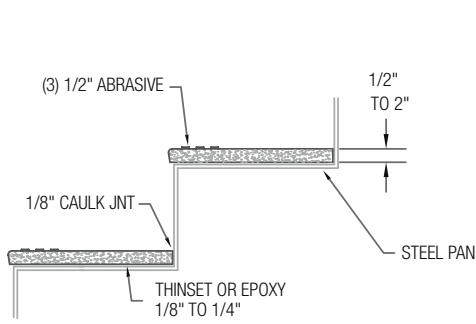
TT2000™ SERIES E-30 FLAT EPOXY TERRAZZO TREAD
