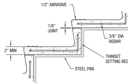
S-36 CEMENT TERRAZZO TREAD AND RISER
