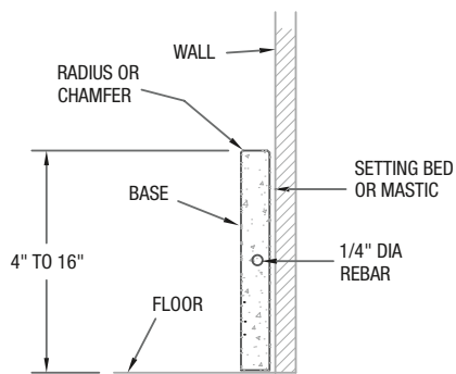
3/4" THICK FLAT CEMENT TERRAZZO BASE
