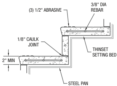
S-40 CEMENT TERRAZZO SEPARATE TREAD AND RISER
