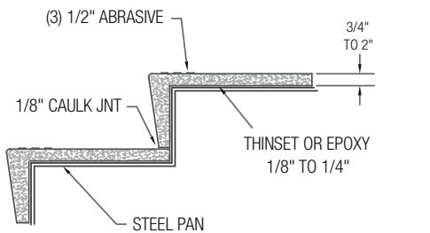
TT2000™ SERIES E-31 EPOXY TERRAZZO TREAD AND RISER
