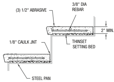
S-30 CEMENT TERRAZZO TREAD
