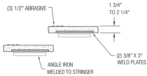
TT2000™ SERIES ESS-30 FLAT EPOXY TERRAZZO SELF-SUPPORTING TREAD
