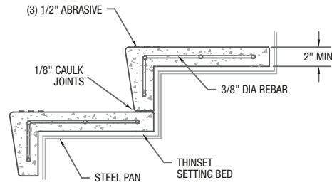
S-31 CEMENT TERRAZZO TREAD AND RISER
