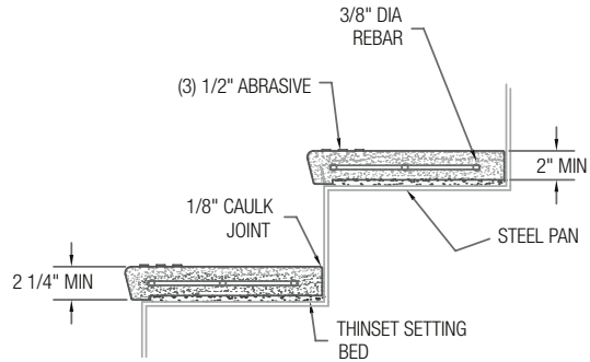
EC-30 FLAT EPOXY TERRAZZO TREAD
