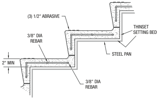
S-41 CEMENT TERRAZZO TREAD AND RISER
