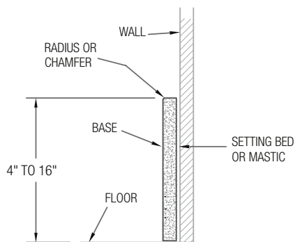
3/8" THICK FLAT EPOXY TERRAZZO BASE
