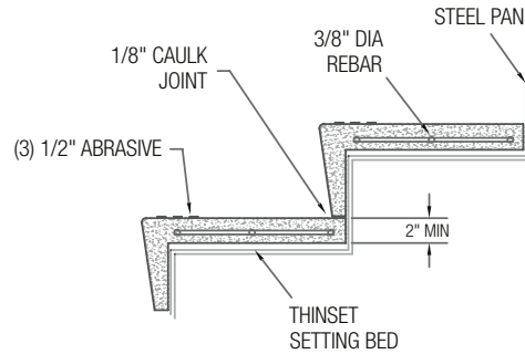
EC-31 EPOXY TERRAZZO TREAD & RISER
