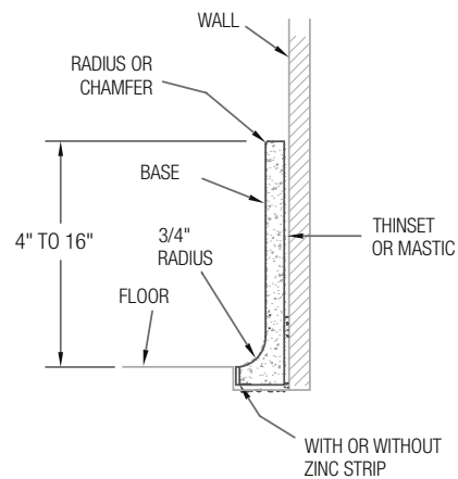
3/8" THICK COVERED EPOXY TERRAZZO BASE
