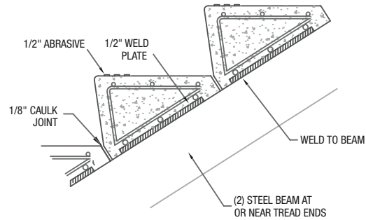
CUSTOM SELF-SUPPORTING TRIANGULAR CEMENT TERRAZZO TREAD
