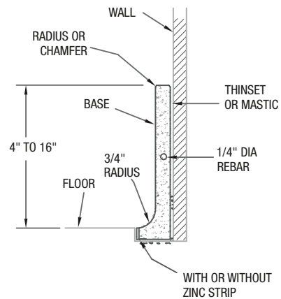
3/4" THICK COVERED CEMENT TERRAZZO BASE
