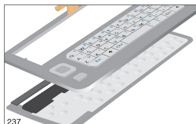
237 With differential adhesive, the silicone adhesive side of 3M™ Double Coated Tape adheres to a silicone rubber keypad. Acrylic adhesive side adheres to a plastic base.
