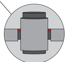
3M™ Fire Barrier Sealant CP 25 WB+ & Packing Material PM 4 C-AJ-5210
