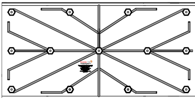
UNDERSIDE VIEW
