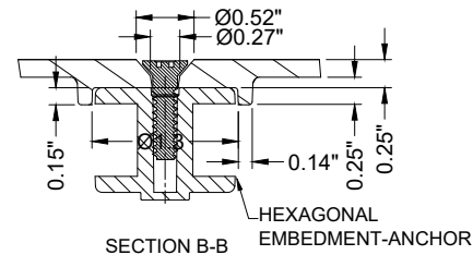
SECTION B-B HEXAGONAL EMBEDMENT-ANCHOR
