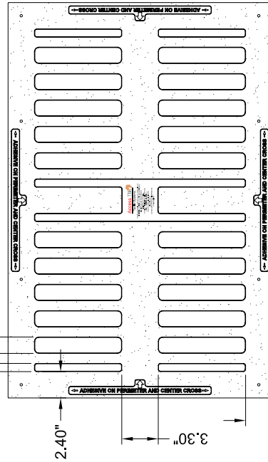
UNDERSIDE VIEW
