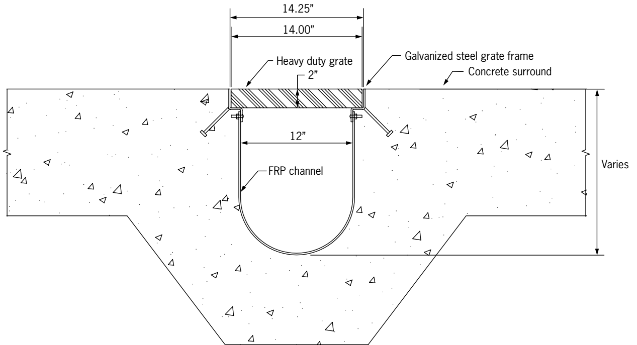
Aquaduct 12" Custom Trench Drain (NTS)
