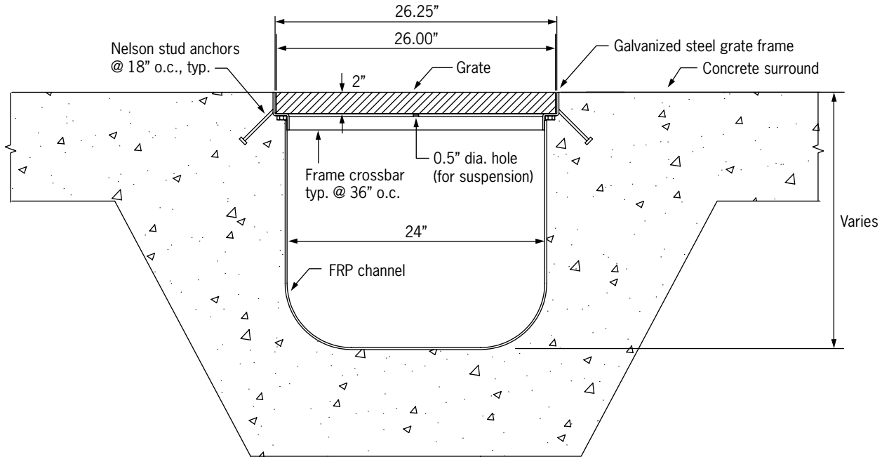
Aquaduct 24" Custom Trench Drain (NTS)
