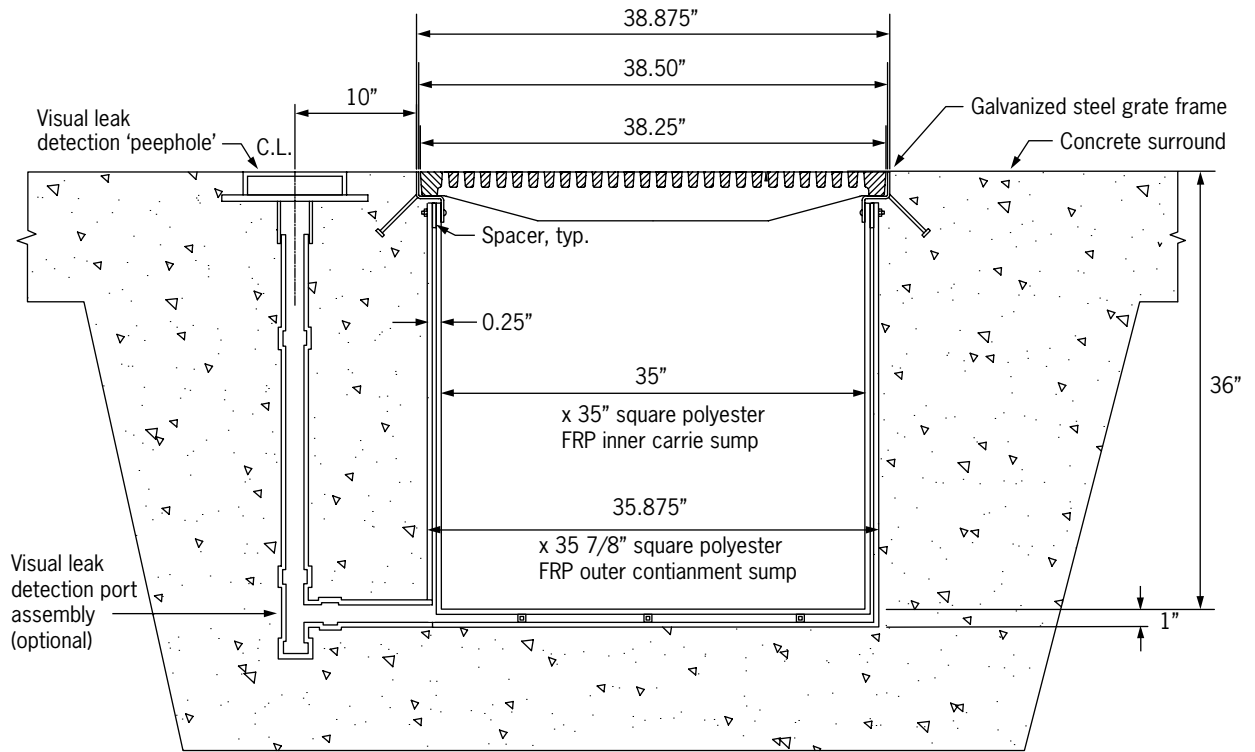
Typical Aquaduct Custom Double Containment Sump (NTS)
