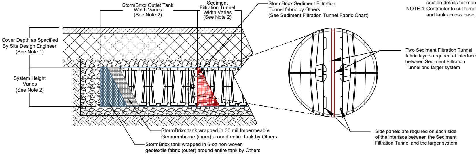
SYSTEM CROSS SECTION
