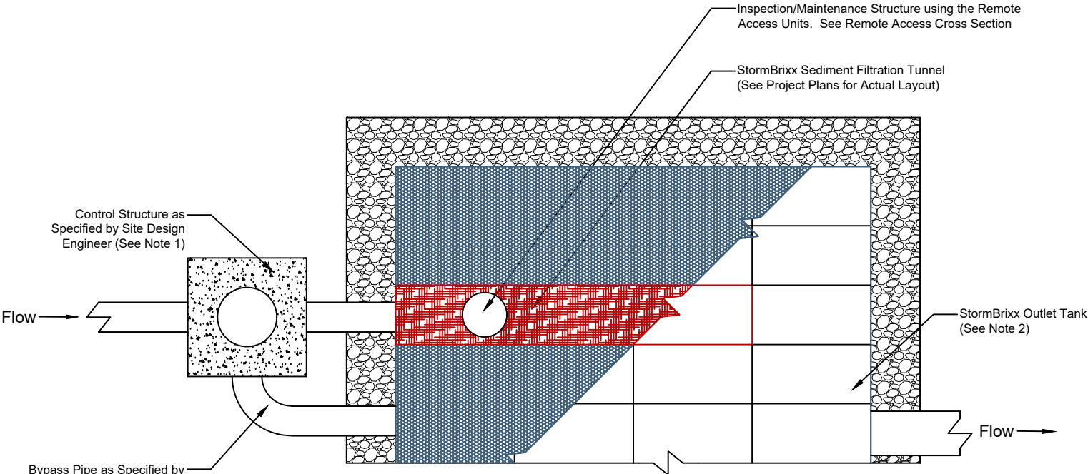
STORMBRIXX SEDIMENT FILTRATION TUNNEL EXAMPLE LAYOUT
