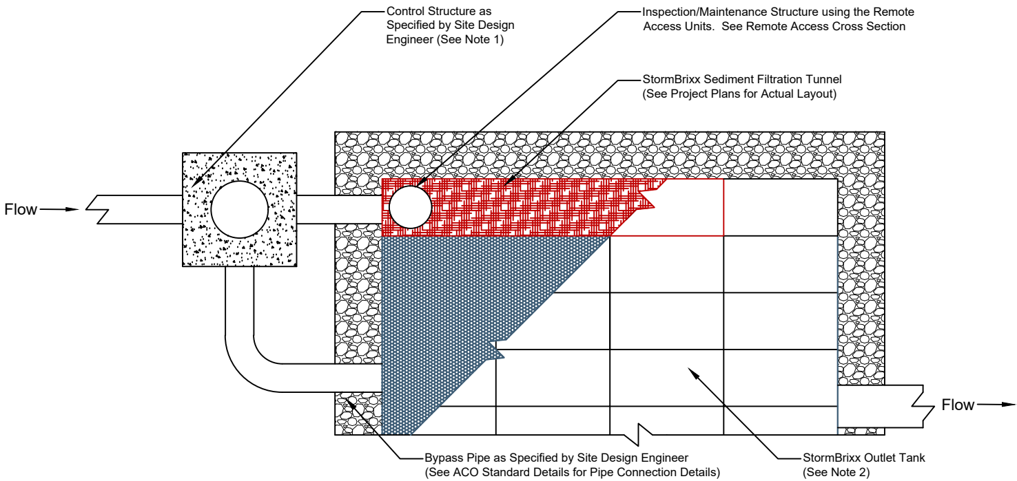
STORMBRIXX SEDIMENT FILTRATION TUNNEL EXAMPLE LAYOUT
