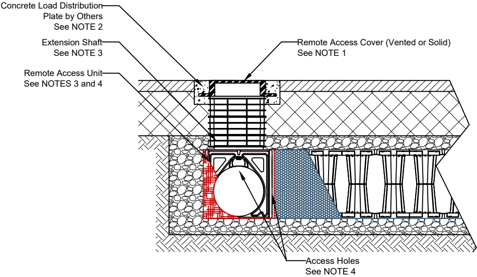
ACCESS POINT CROSS SECTION
