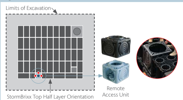
Figure 5: Module Install Plan View
