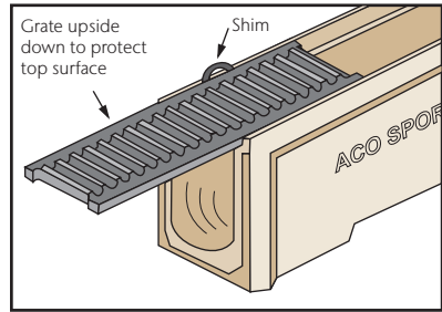
System 4000 Bracing
