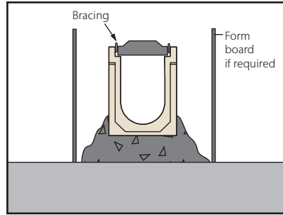
System 4000 Bracing
