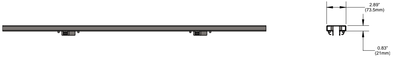
Side elevation
