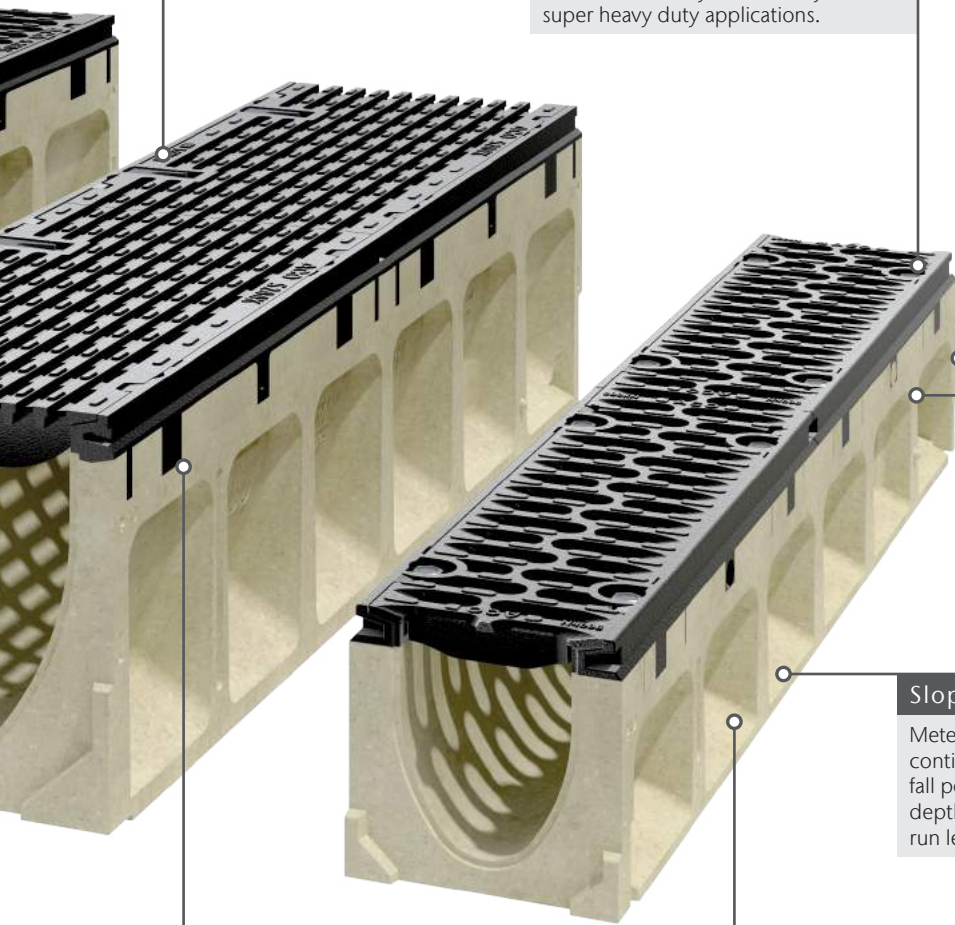
Profiled Side Walls Strengthening pillars and frost keys provide channel body strength and mechanical keying to surrounding concrete.
