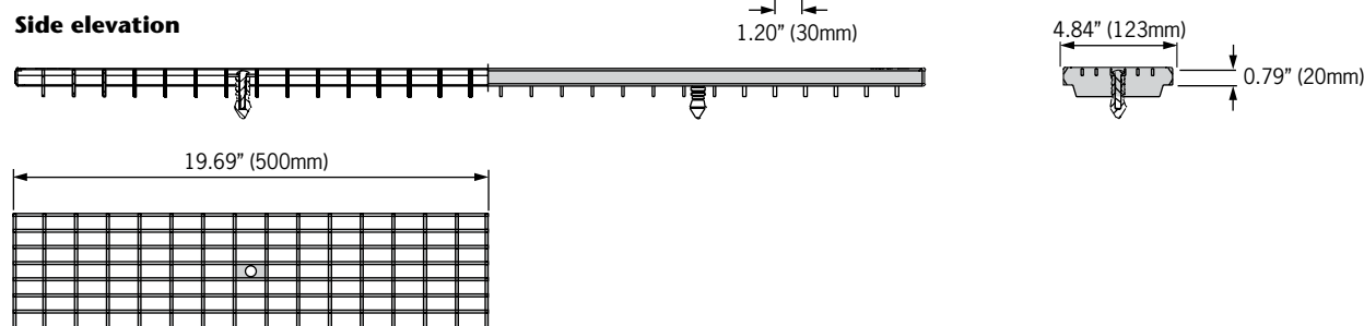
Side elevation
