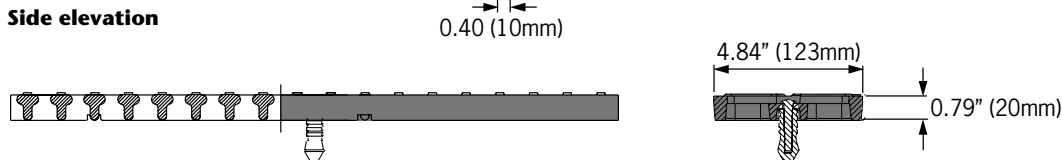
Side elevation
