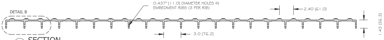
CC SECTION
