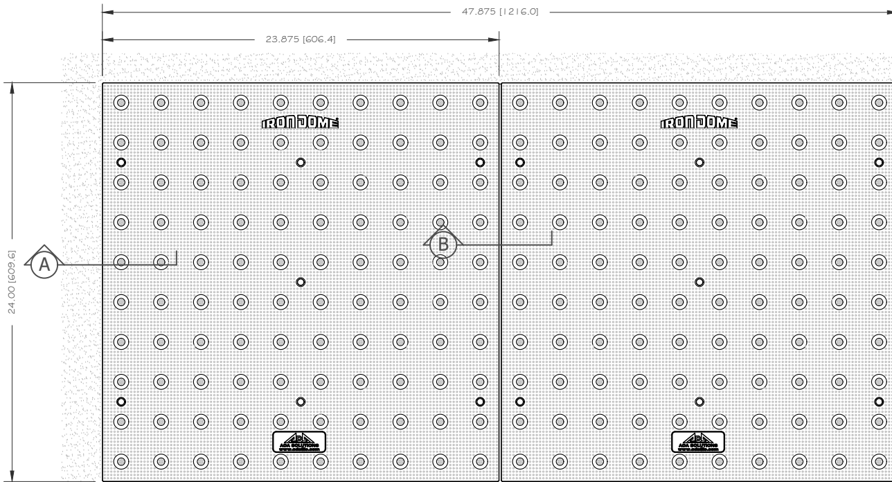
TOP VIEW - MULTIPLE PANEL INSTALLATION (2 PANELS)
