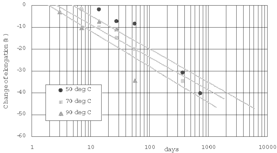
Fig.1) Relationship between change of elongation and days
