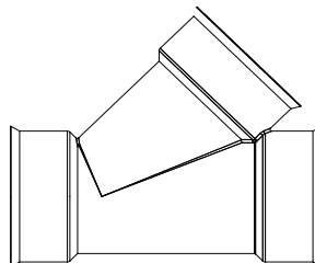
SIZE-ON-SIZE OR REDUCING 45-DEG WYE
