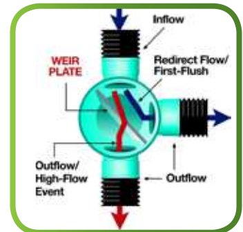
WEIR STRUCTURE
