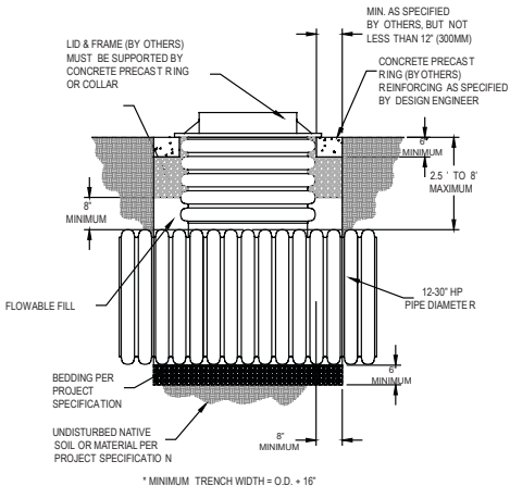
Figure 6: Vertical Riser
