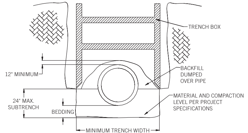
Figure 2: Subtrench Installation
