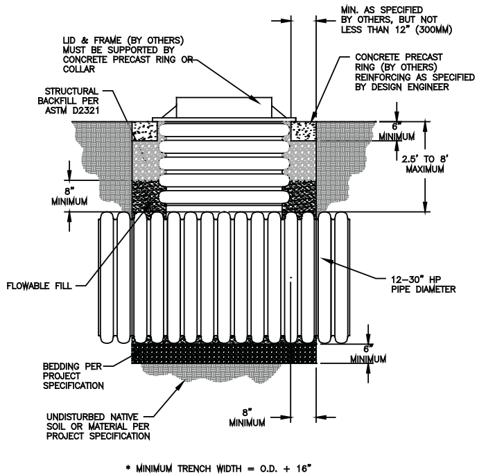
Figure 6: Vertical Riser
