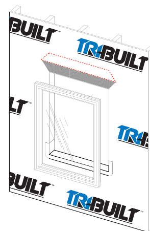
Figure 5: Window installation in accordance with window manufacturer's instructions.
