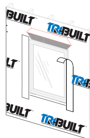
Figure 6: Flashing applied to jambs.
