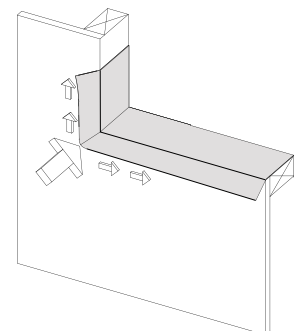
Figure 4: Direction of application of flexible flashing at sill and jamb intersection.
