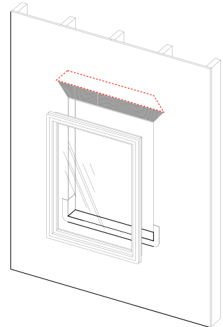
Figure 5: Window installation in accordance with window
