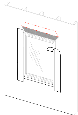
Figure 6: Flashing applied to jambs.
