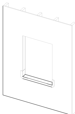
Figure 4: Direction of application of flexible flashing at sill and jamb intersection.
