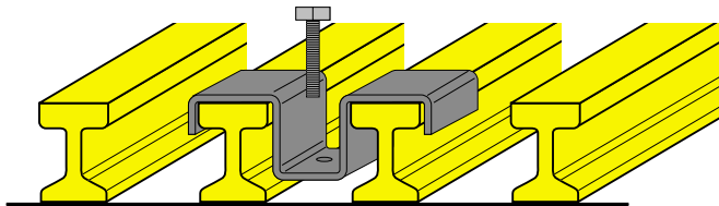
316 stainless steel alloy for I-50, I-60, and T-50 series grating
