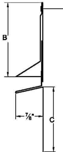
M-SLIDE HORIZONTAL EXPANSION JOINT SECTION VIEW
