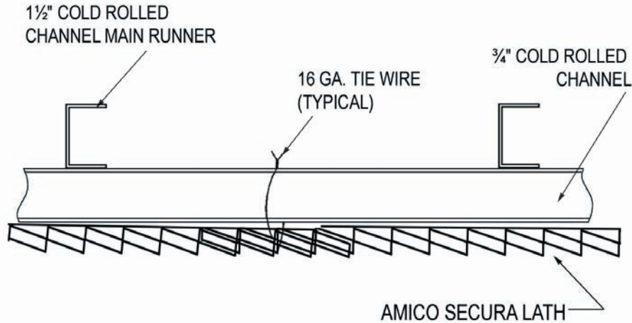
TYPICAL LAP JOINT WIRE-TIED
