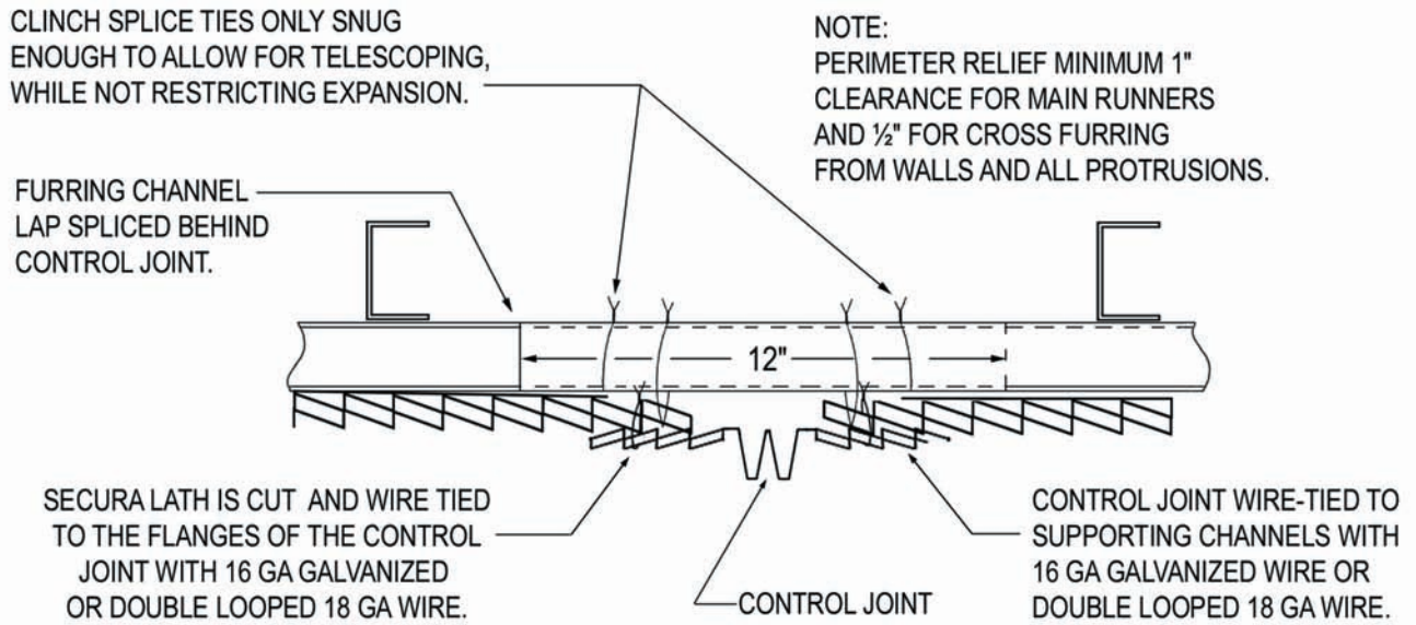
CONTROL JOINT PERPENDICULAR TO FURRING CHANNEL
