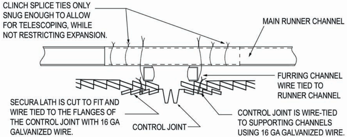
CONTROL JOINT PARALLEL TO FURRING CHANNEL
