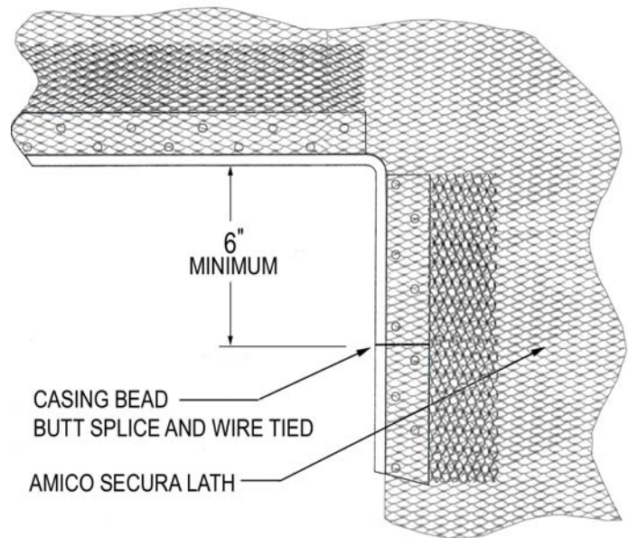
TYPICAL CEILING OPENING
