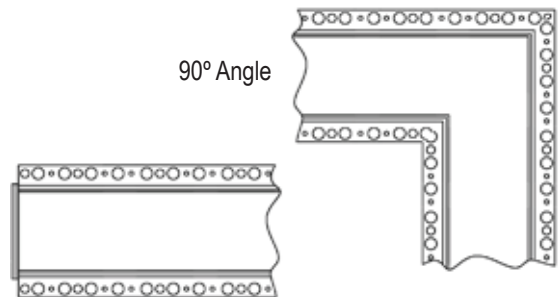
End Closure
