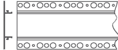
CAD Detail Name: Vinyl Stucco Reveal Click Link to go to Print Details
