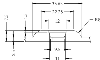
SECTION B-B CONCEALED MECHANICAL FASTENING
