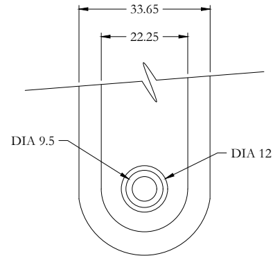
DETAIL 1
