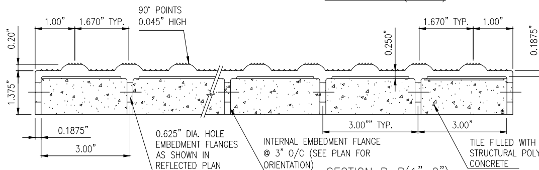
SECTION B-B (1"=2")
